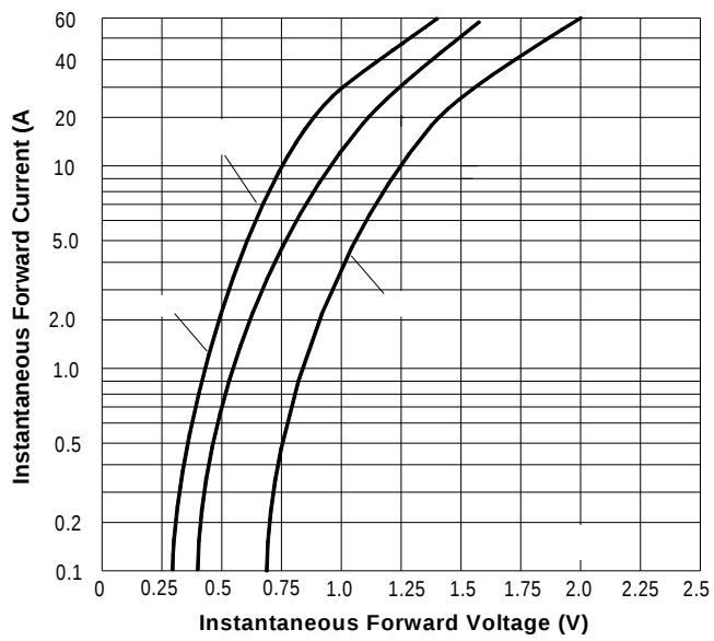
FIG3: Forward Voltage
